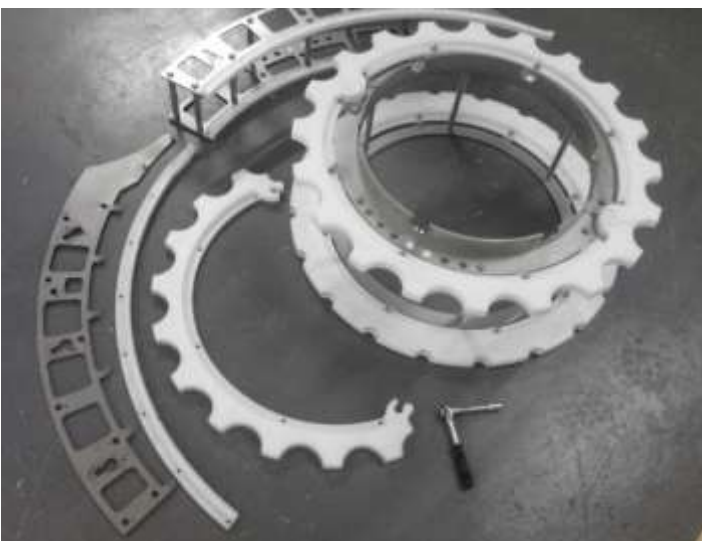
Bottling Star Wheel Laser Profiling
